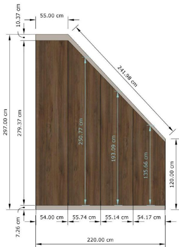
0 Front view Scale: 0" : 0"
