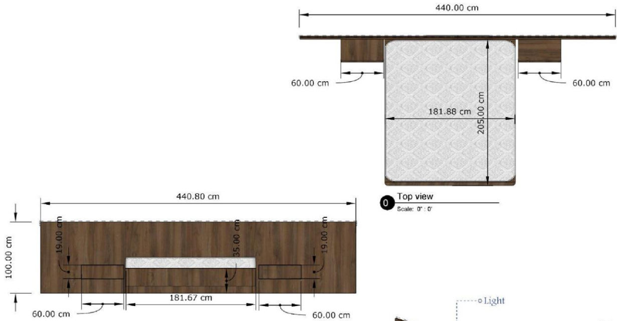
0 Front view Scale: 0" : 0"
