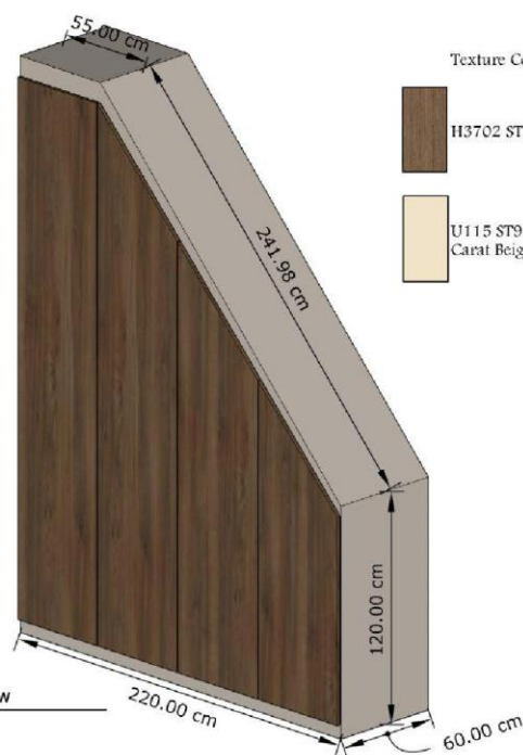
0 Isometric view Scale: 0" : 0"
